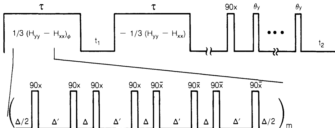
Figure 4. Two-dimensional multiple-quantum pulse sequence for solids. The preparation and mixing periods are composed of eight \pi/2 pulses of length t_p ( =2.5 \mu\text{s} ) separated by delays \Delta ( =2.5 \mu\text{s} ) and \Delta' ( =7.5 \mu\text{s} ). The total preparation/mixing time \tau is achieved by repeating the basic 60- \mu\text{s} cycle m times. When the phases of the pulses are x and \bar{x} , the Hamiltonian is equal to 1/3(H_{yy} - H_{xx}) ; during the mixing period, when the phases of the pulses are y and \bar{y} , the Hamiltonian becomes -1/3(H_{yy} - H_{xx}) , i.e., the negative of the preparation period Hamiltonian. To separate the multiple-quantum orders, the preparation period pulses are incremented by a phase \phi for each value of t_1 . During the detection period, a pulsed spin-locking sequence is used for signal enhancement in samples containing low ^1\text{H} concentrations.
