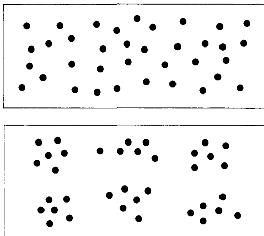
Figure 1. Possible atomic distributions in solids. Uniform and clustered distributions can be distinguished by time-resolved solid-state multiple-quantum NMR.
