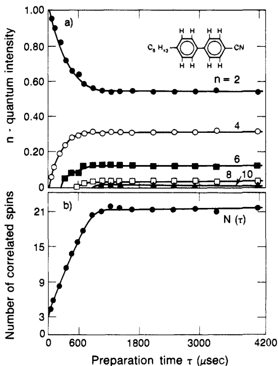
Figure 6. (a) n -Quantum intensity vs. preparation time for the liquid crystal, p -hexyl- p' -cyanobiphenyl in the nematic phase. The intensity of each multiple-quantum order has been normalized to the two-quantum intensity, and smooth curves have been drawn through the data points to aid the eye. From top to bottom, n = 2 corresponds to filled circles; n = 4 to open circles; n = 6 to filled squares; n = 8 to open squares; n = 10 to filled triangles. After roughly 1000 \mu\text{s} , no new multiple-quantum orders develop and their relative intensities remain unchanged. (b) N(\tau) vs. \tau for the liquid crystal sample. After an induction period, the effective system size N(\tau) levels off at 21, indicating that the number of interacting spins is limited to the size of the individual liquid crystal molecules which contain 21 protons.
