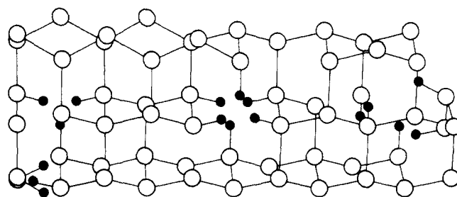
Figure 13. Schematic three-dimensional drawing of clustered mono-hydrides in hydrogenated amorphous silicon (a-Si:H). The silicon atoms are in a tetrahedral bonding configuration. Silicon atoms, hydrogen atoms, and covalent bonds are represented by open circles, filled circles, and solid lines, respectively. The drawing is intended to motivate questions concerning the distribution of hydrogen in a-Si:H thin films.
