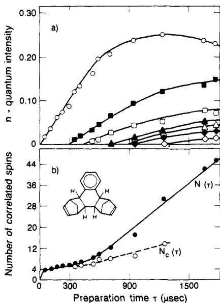
Figure 12. (a) n -Quantum intensity vs. preparation time for the polycrystalline sample 1,2,3,4-tetrachloronaphthalene-bis(hexachlorocyclopentadiene) adduct. The two-quantum intensity is not plotted so that higher multiple-quantum orders can be seen more clearly. The time development of the multiple-quantum intensities is discontinuous. (b) Number of correlated spins vs. preparation time for this sample. The effective system size N(\tau) remains at 4 for times up to 300 \mu\text{s} , indicating that only the four hydrogen atoms within the molecule have become correlated thus far. At long times, a large number of intercluster interactions can develop.
