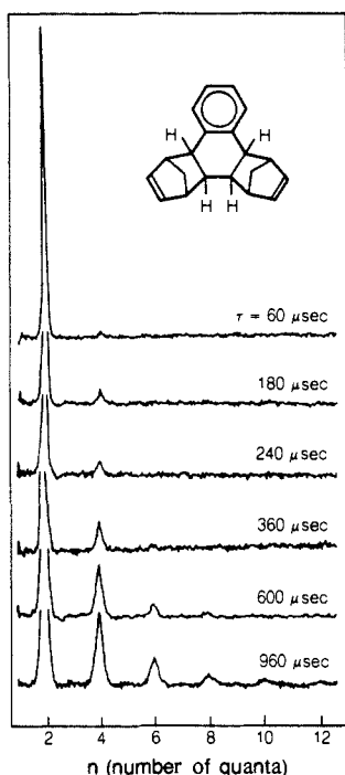
Figure 2. ^1\text{H} multiple-quantum (180-MHz) NMR spectra of the polycrystalline sample 1,2,3,4-tetrachloronaphthalene-bis(hexachlorocyclopentadiene) adduct. The time development of the multiple-quantum coherences is discontinuous in this clustered material. The spectra change very little over the first 300 \mu\text{s} , indicating a limited spin system on this time scale. At longer times, when intermolecular interactions develop, the system is no longer bounded and higher multiple-quantum orders arise in the spectrum.
